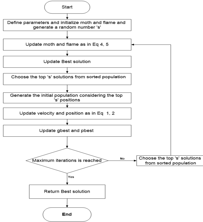
Figure 1: MFO_PSO flowchart
