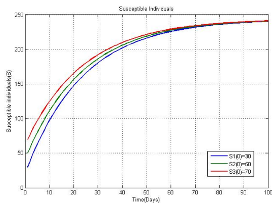
Figure 2: Susceptible individuals.
