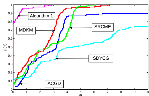
Figure 3: Dolan and More profile for CPU time
