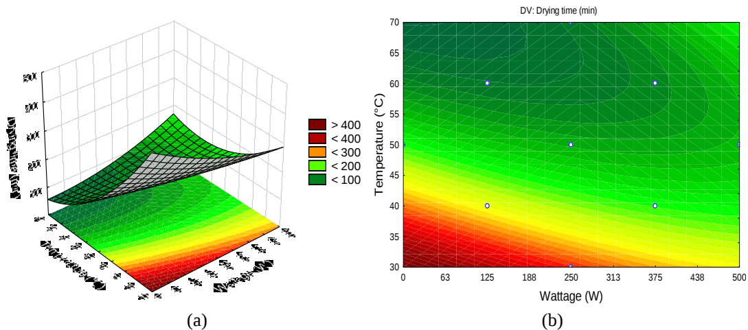
Fig. 11. (a) Response surface and (b) contour of the drying time of red seaweed ( Chondracanthus chamissoi ) for the independent variables of drying air temperature and incandescent lamp wattage, keeping the critical values of load density and drying air velocity fixed
