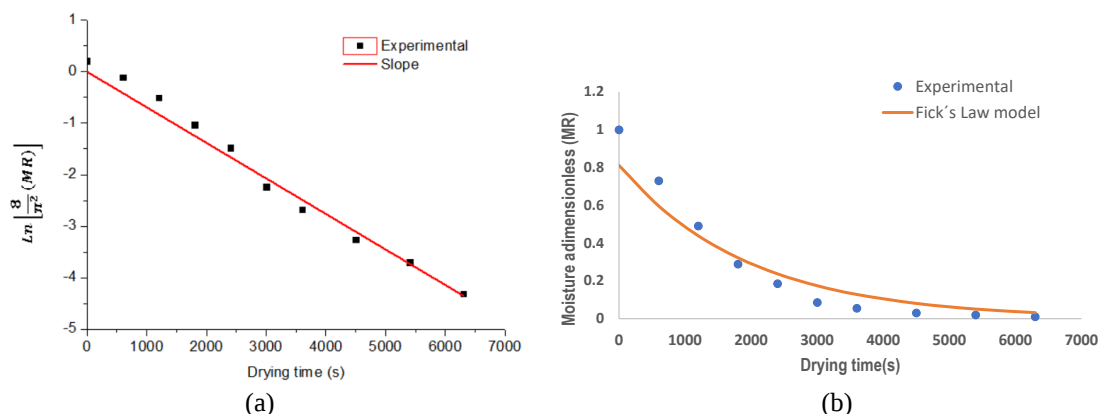
Fig. 13. (a) Determination of the slope for the calculation of diffusivity; (b) Drying curve and simulation with the Fick equation of red seaweed ( Chondracanthus chamissoi )
