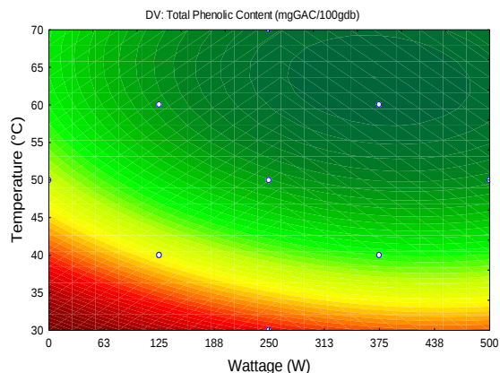
Fig. 7. (a) Response surface and (b) contour of the total phenolic content (mg GAC/100 g db ) of red seaweed ( Chondracanthus chamissoi ) dried with hot air assisted by incandescent lamps
