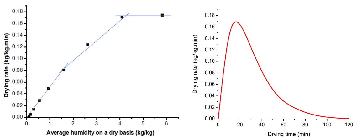
Fig. 15. Red seaweed drying kinetics
