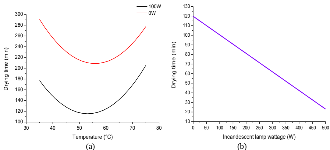
Fig. 12. (a) Behavior of the drying times versus air temperature for two values of the incandescent lamp wattage with constant drying air velocity ( 1.5 \text{ m s}^{-1} ) and charge density ( 4.0 \text{ kg m}^{-2} ); (b) Graphical simulation of the drying times of the red seaweed for variations of the incandescent lamp wattage
