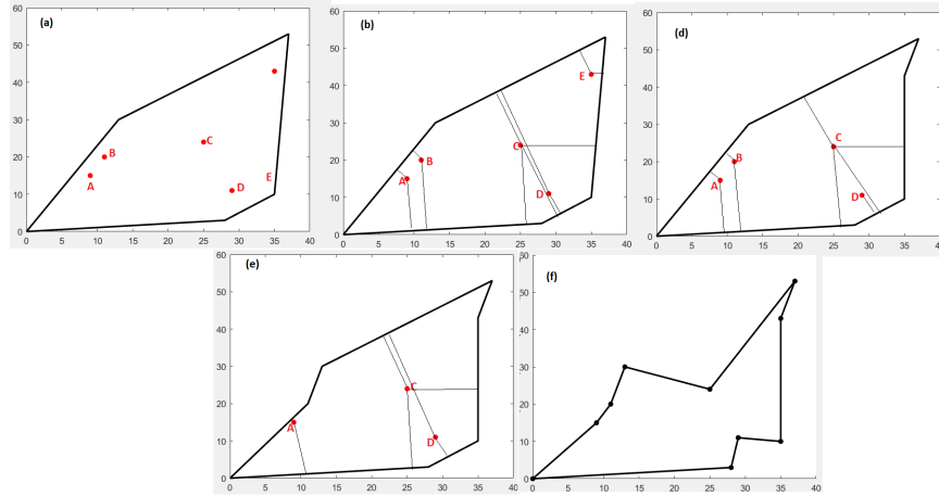
Figure 2: Steps of CH-insertion Algorithm 3
