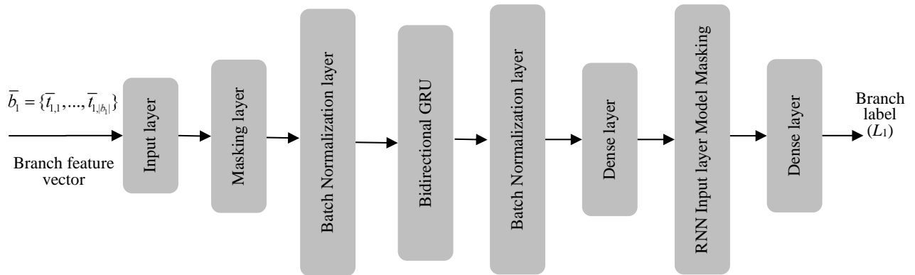
Figure 6. The architecture of the RNN unit
