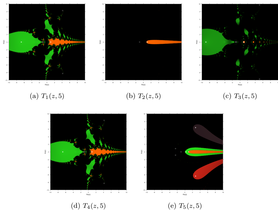
Figure 3: Dynamical planes corresponding to rational operators under study for a = 5 .
