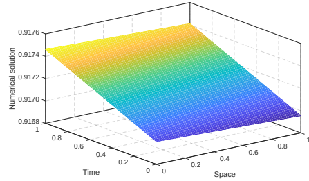
Figure 2: Three-dimensional representation of numerical solution of Example 1 with s = 0.01 , \Delta t = 0.001 , and \sigma = 8 .
